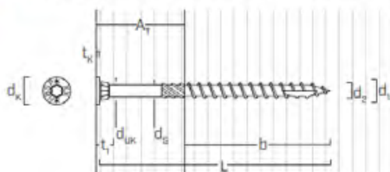
HBS P EVO - 5,0 | 6,0 mm
